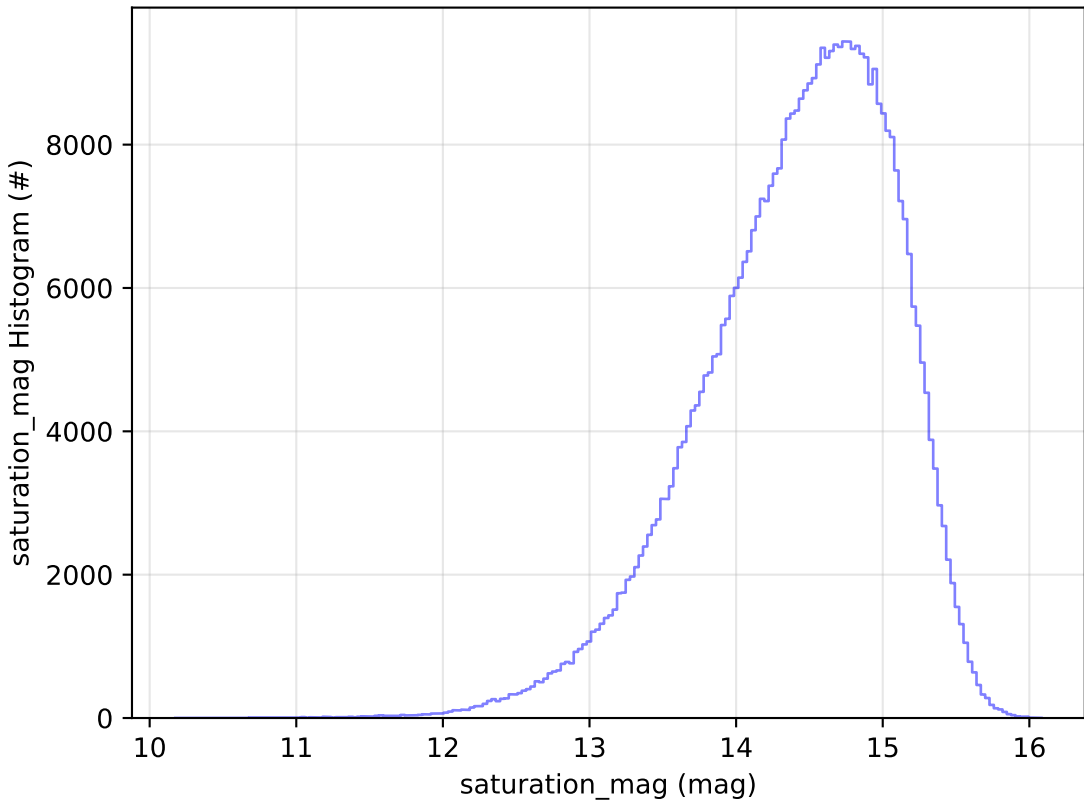
too_elab_r128_d2_gz_v3.4_10yrs All sky i band: saturation_mag Histogram
