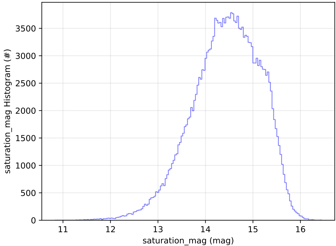
too_elab_r128_d2_gz_v3.4_10yrs All sky g band: saturation_mag Histogram
