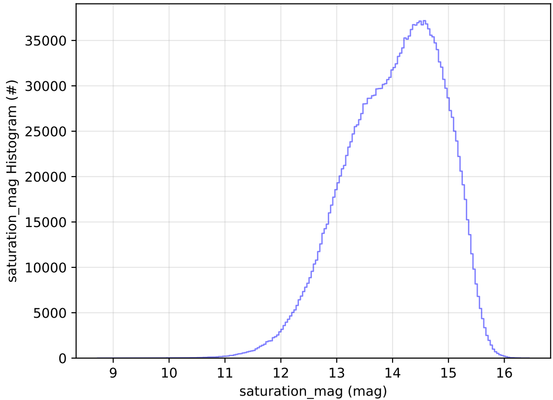
too_elab_r128_d2_gz_v3.4_10yrs All sky all bands: saturation_mag Histogram
