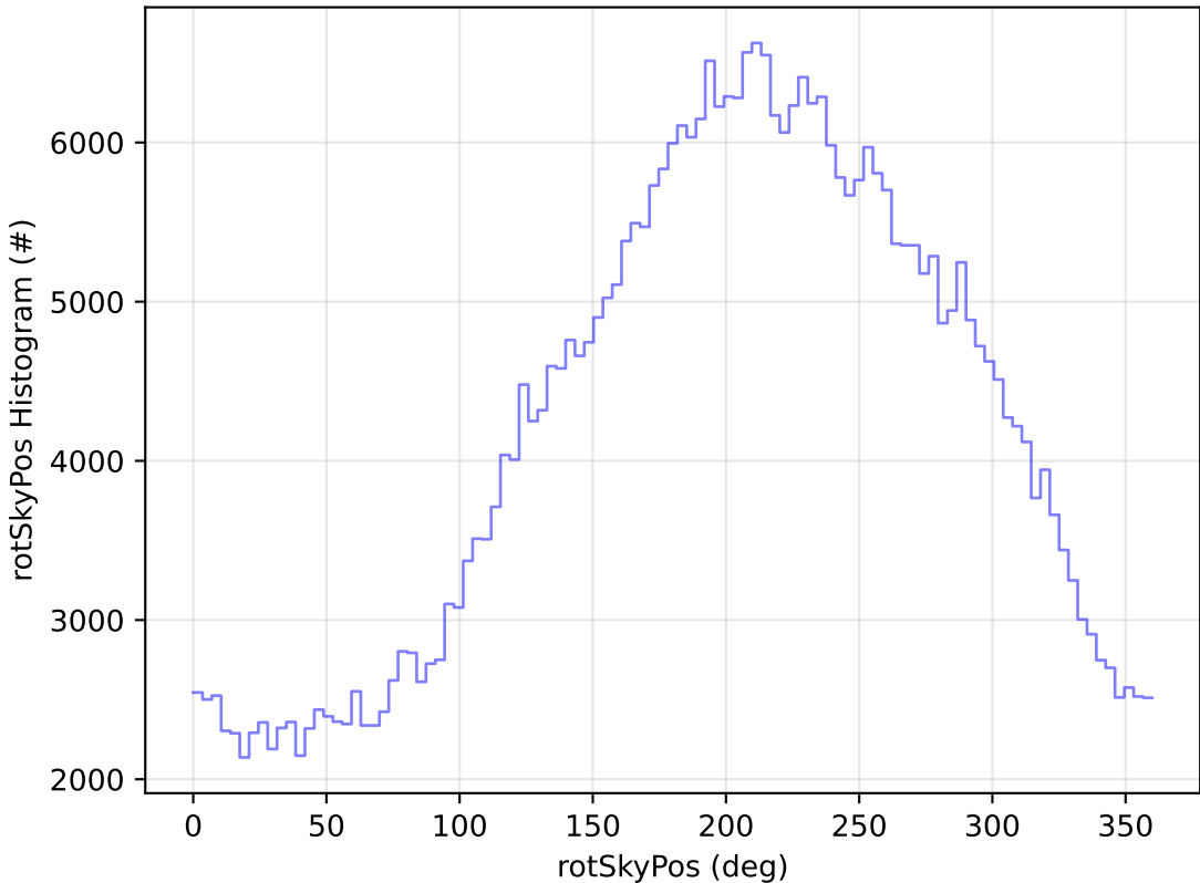
too_elab_r128_d2_gz_v3.4_10yrs WFD z band: rotSkyPos Histogram
