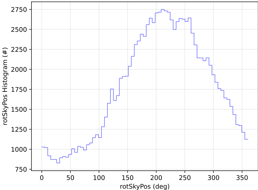
too_elab_r128_d2_gz_v3.4_10yrs WFD u band: rotSkyPos Histogram
