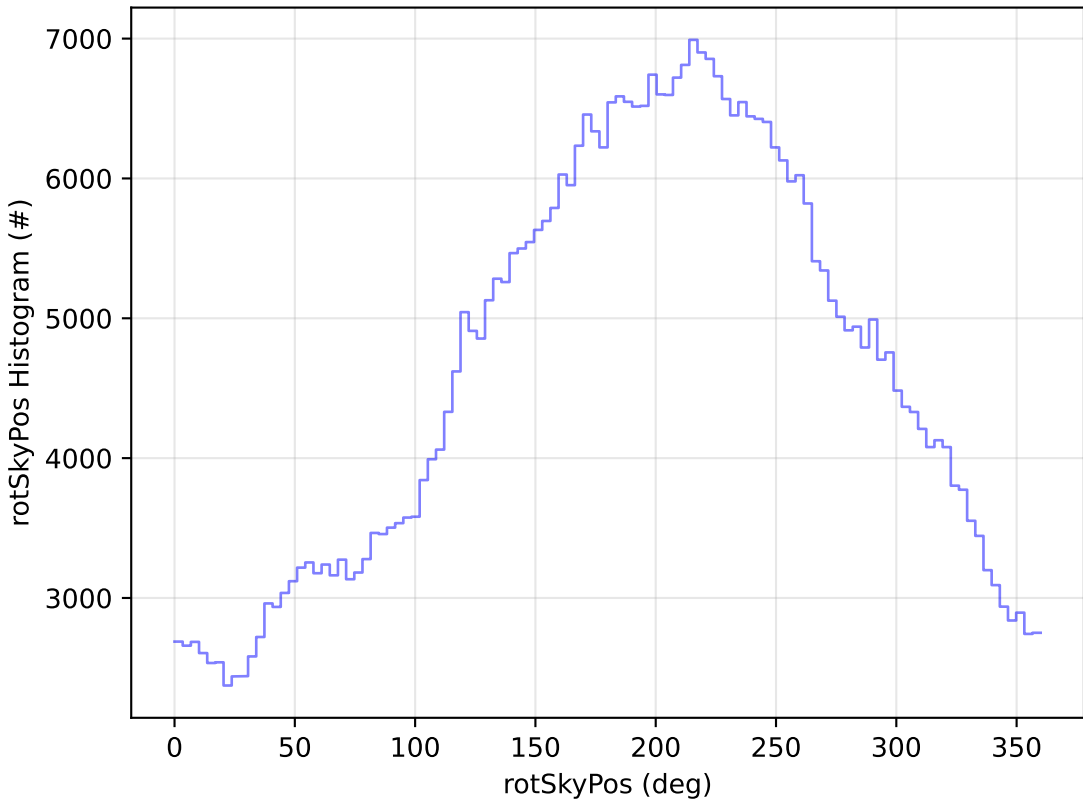
too_elab_r128_d2_gz_v3.4_10yrs WFD r band: rotSkyPos Histogram
