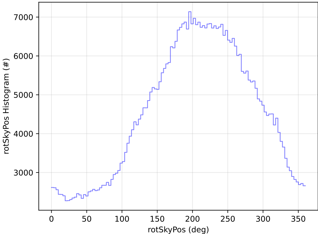
too_elab_r128_d2_gz_v3.4_10yrs WFD i band: rotSkyPos Histogram
