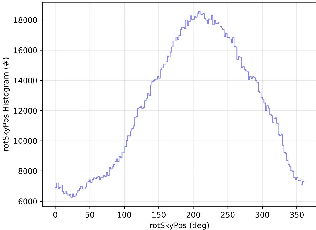
too_elab_r128_d2_gz_v3.4_10yrs WFD all bands: rotSkyPos Histogram
