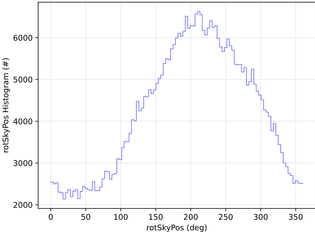
too_elab_r128_d2_gz_v3.4_10yrs All sky z band: rotSkyPos Histogram
