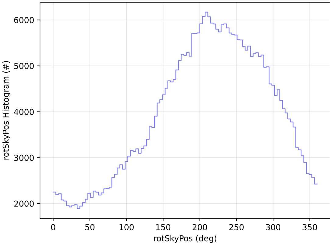
too_elab_r128_d2_gz_v3.4_10yrs All sky y band: rotSkyPos Histogram
