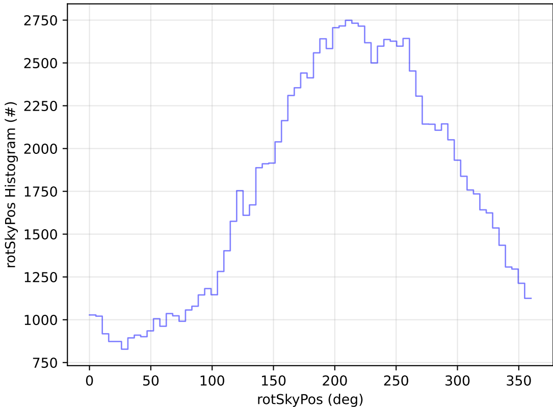
too_elab_r128_d2_gz_v3.4_10yrs All sky u band: rotSkyPos Histogram
