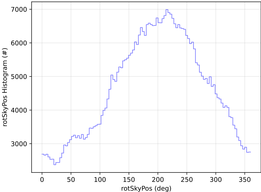
too_elab_r128_d2_gz_v3.4_10yrs All sky r band: rotSkyPos Histogram
