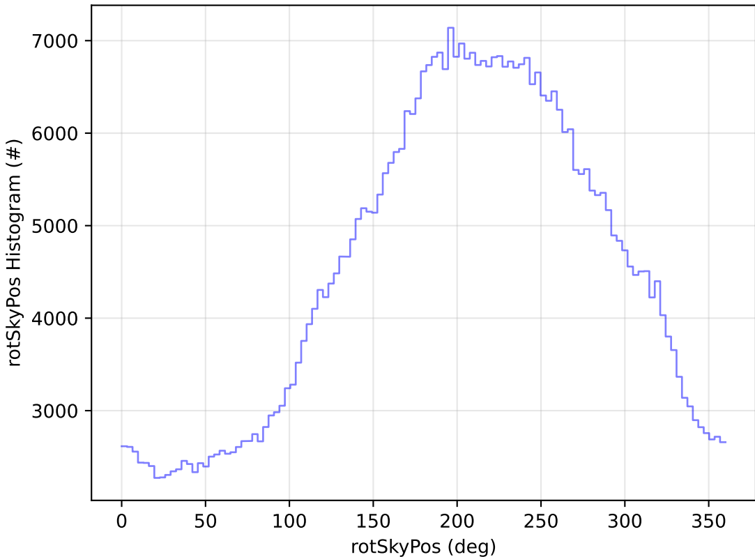
too_elab_r128_d2_gz_v3.4_10yrs All sky i band: rotSkyPos Histogram
