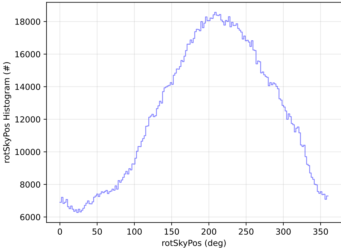
too_elab_r128_d2_gz_v3.4_10yrs All sky all bands: rotSkyPos Histogram
