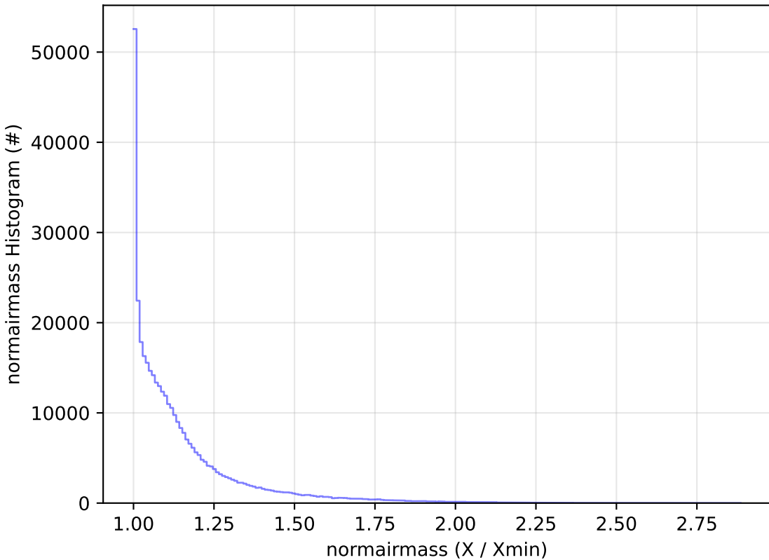
too_elab_r128_d2_gz_v3.4_10yrs WFD y band: normairmass Histogram
