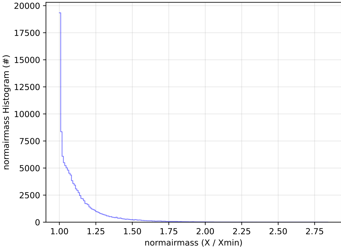
too_elab_r128_d2_gz_v3.4_10yrs WFD u band: normairmass Histogram
