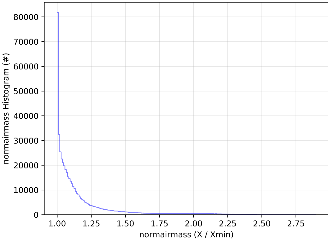
too_elab_r128_d2_gz_v3.4_10yrs WFD r band: normairmass Histogram
