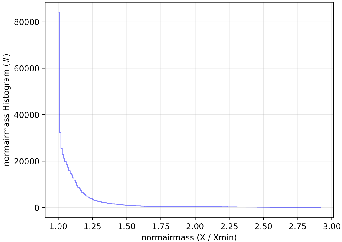
too_elab_r128_d2_gz_v3.4_10yrs WFD i band: normairmass Histogram
