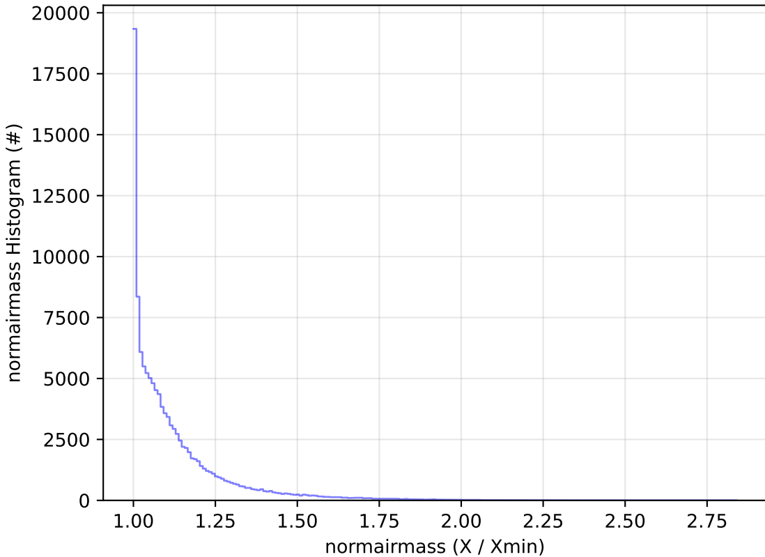
too_elab_r128_d2_gz_v3.4_10yrs All sky u band: normairmass Histogram
