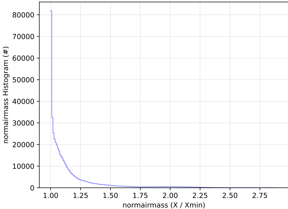
too_elab_r128_d2_gz_v3.4_10yrs All sky r band: normairmass Histogram
