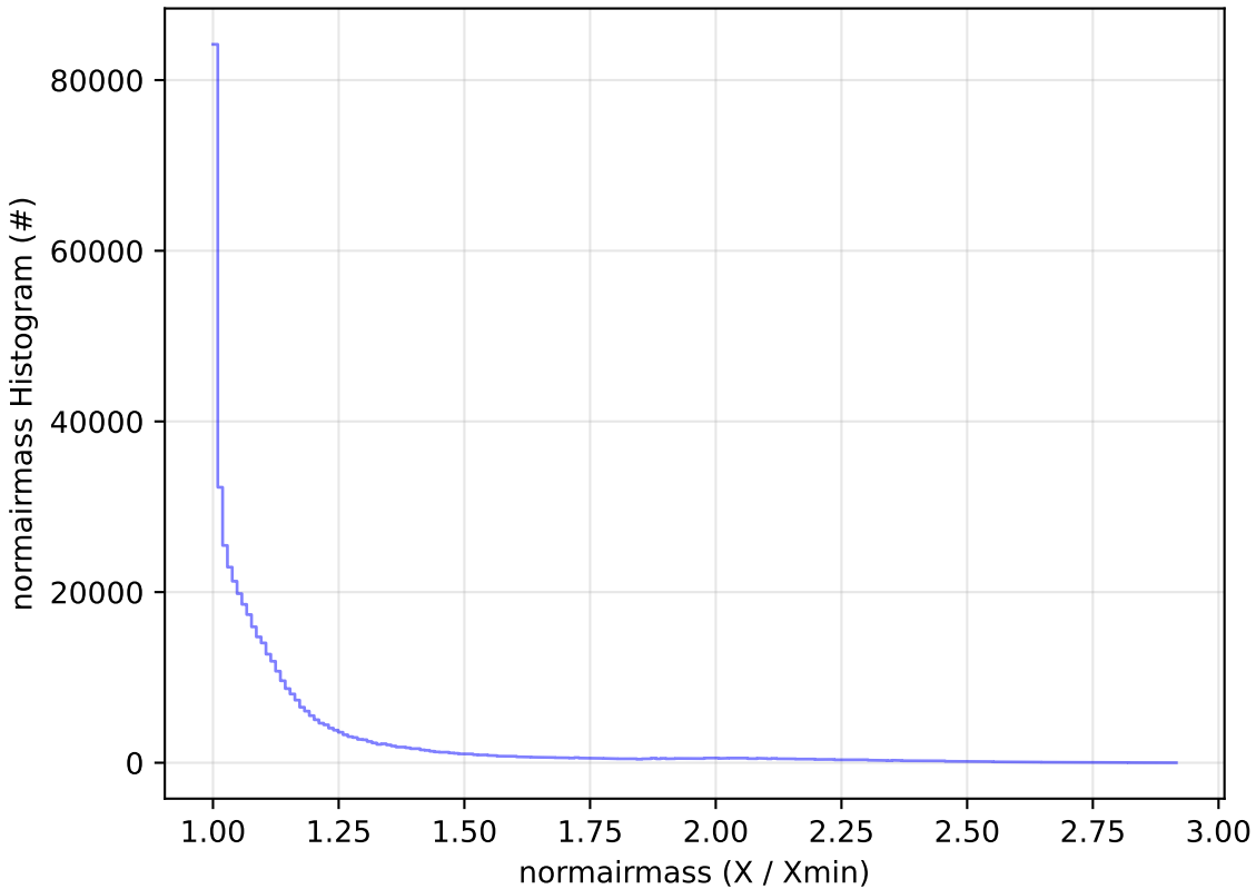
too_elab_r128_d2_gz_v3.4_10yrs All sky i band: normairmass Histogram
