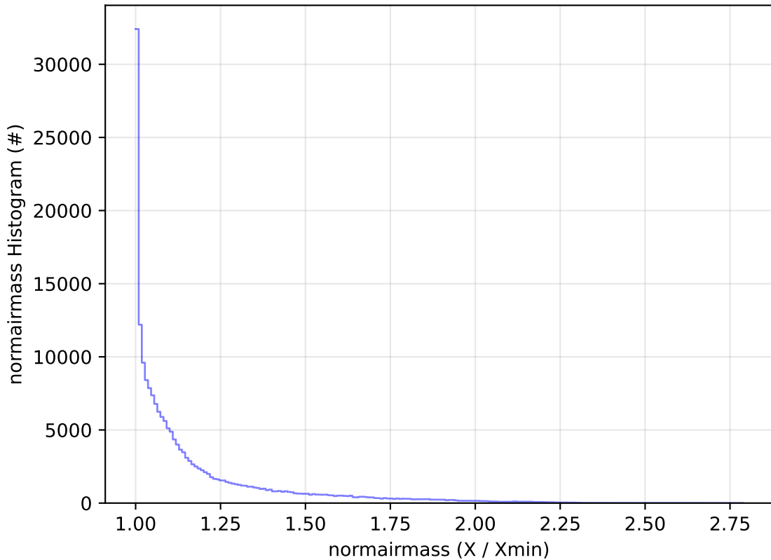
too_elab_r128_d2_gz_v3.4_10yrs All sky g band: normairmass Histogram
