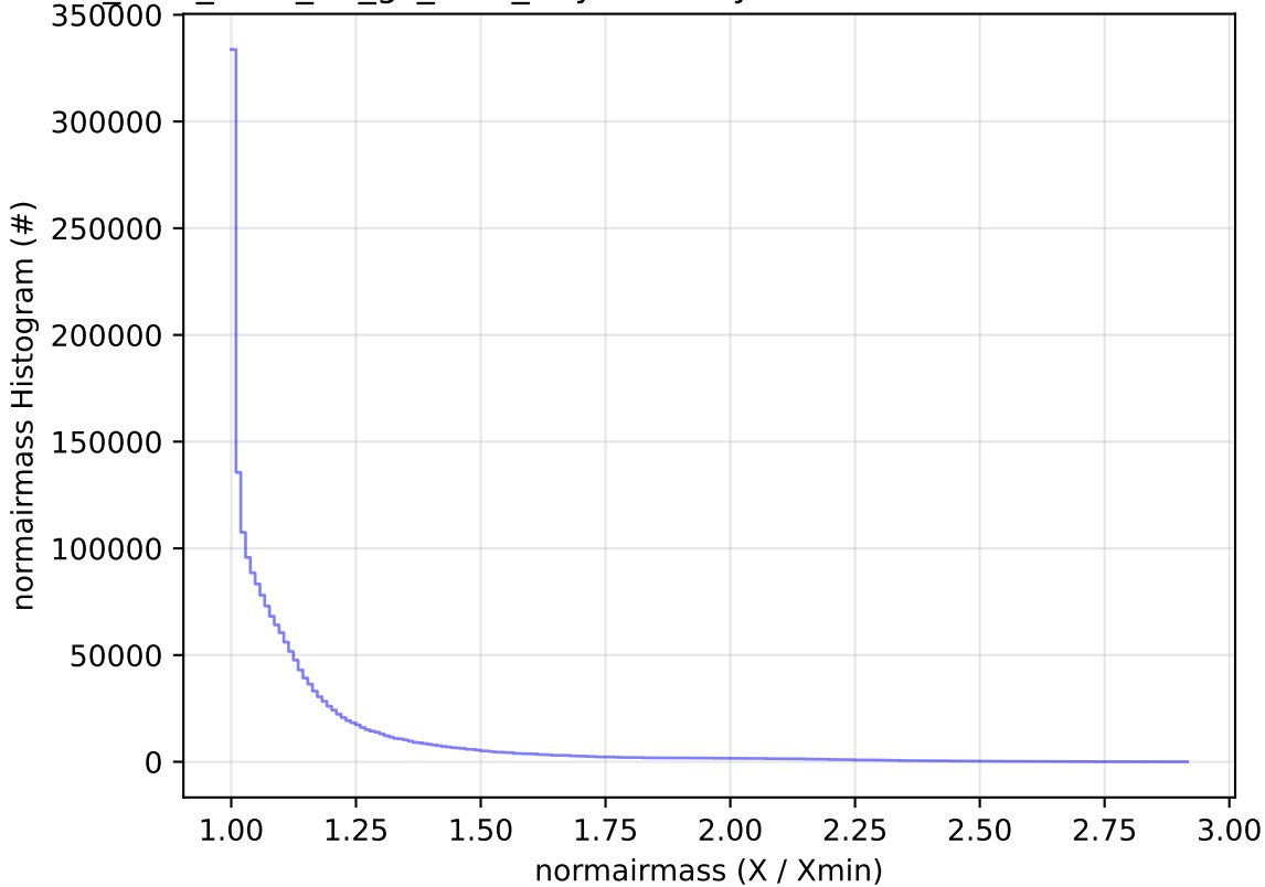
too_elab_r128_d2_gz_v3.4_10yrs All sky all bands: normairmass Histogram
