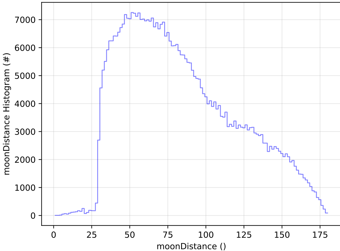
too_elab_r128_d2_gz_v3.4_10yrs WFD z band: moonDistance Histogram
