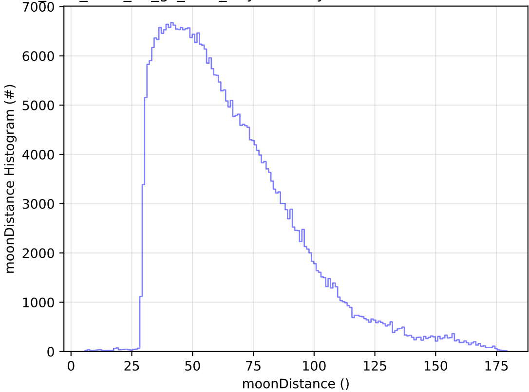
too_elab_r128_d2_gz_v3.4_10yrs WFD y band: moonDistance Histogram
