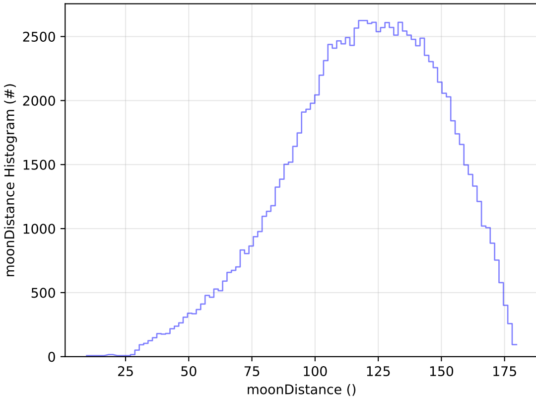
too_elab_r128_d2_gz_v3.4_10yrs WFD u band: moonDistance Histogram
