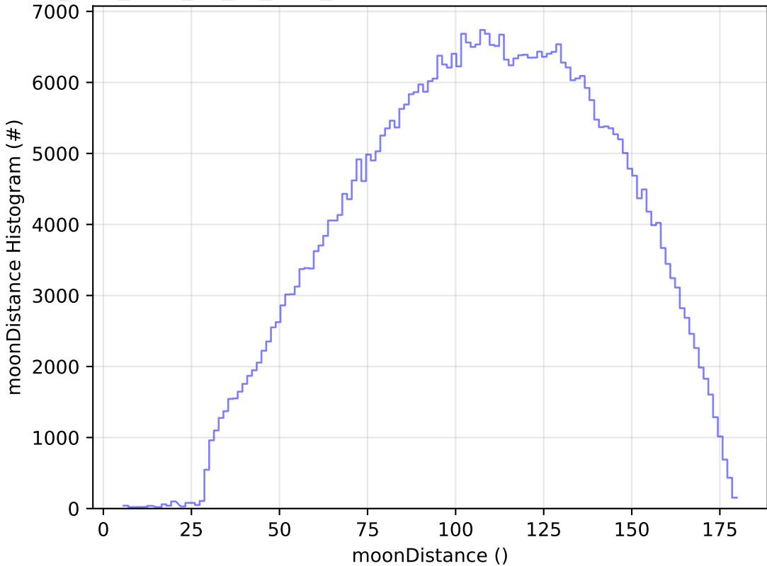
too_elab_r128_d2_gz_v3.4_10yrs WFD r band: moonDistance Histogram
