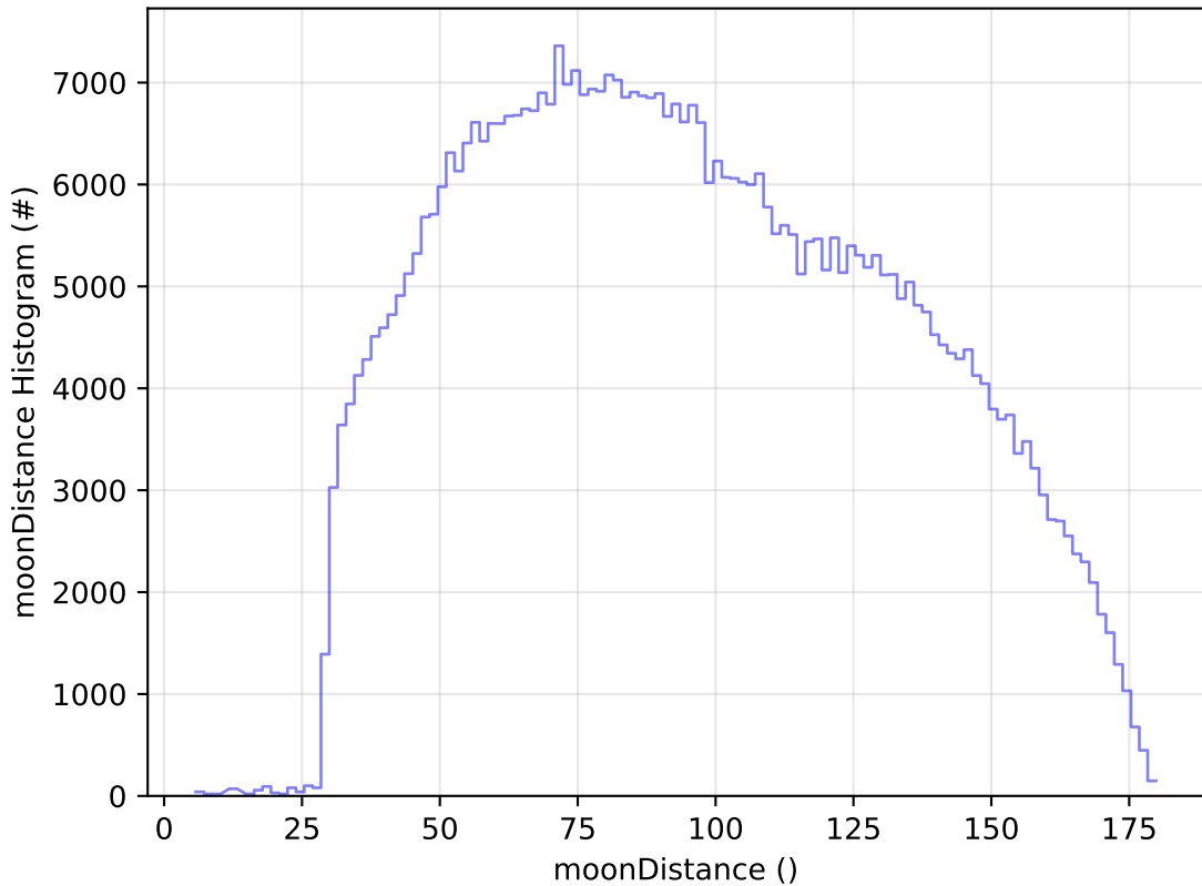
too_elab_r128_d2_gz_v3.4_10yrs WFD i band: moonDistance Histogram
