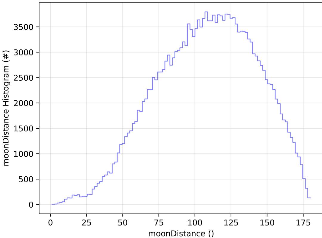
too_elab_r128_d2_gz_v3.4_10yrs WFD g band: moonDistance Histogram
