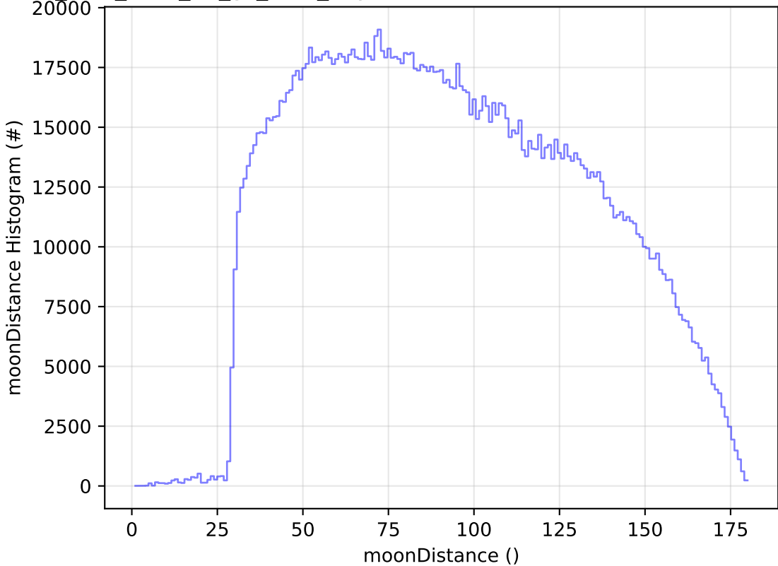
too_elab_r128_d2_gz_v3.4_10yrs WFD all bands: moonDistance Histogram
