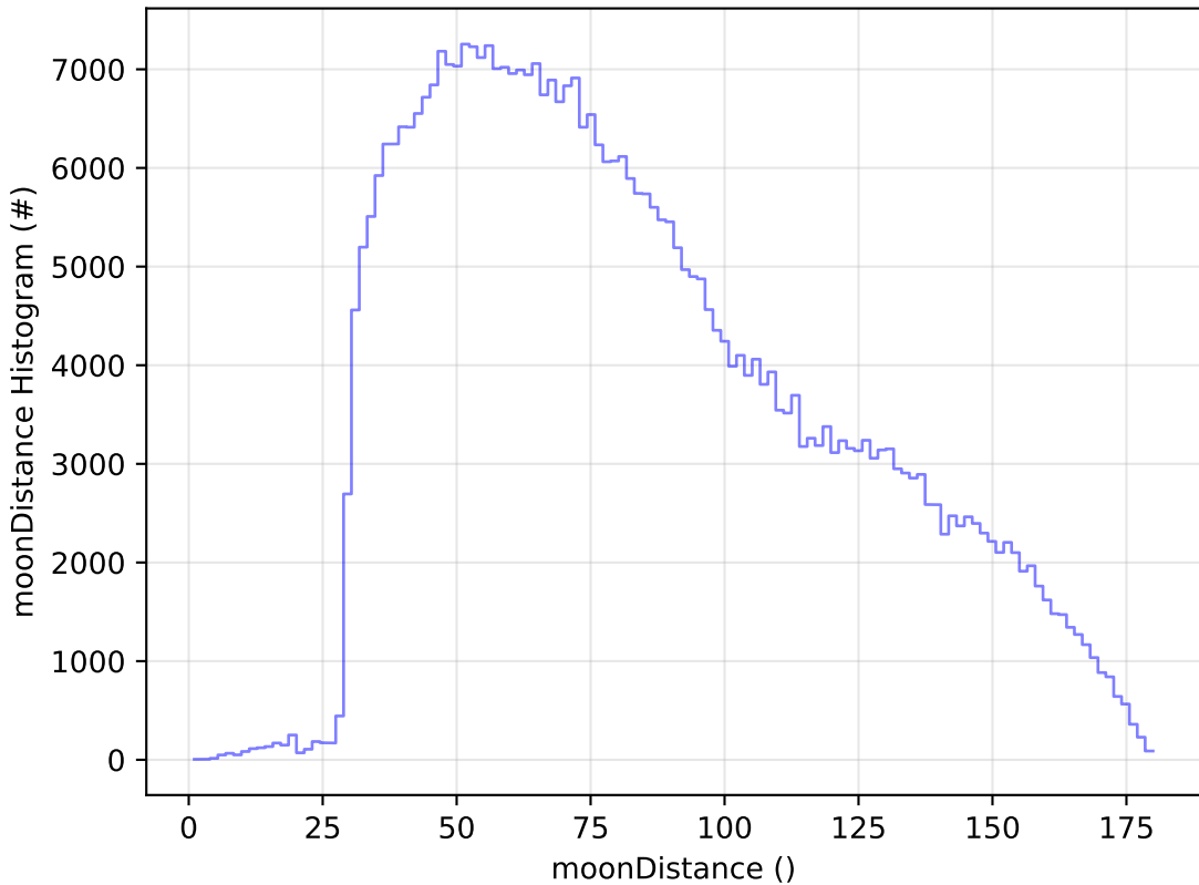
too_elab_r128_d2_gz_v3.4_10yrs All sky z band: moonDistance Histogram
