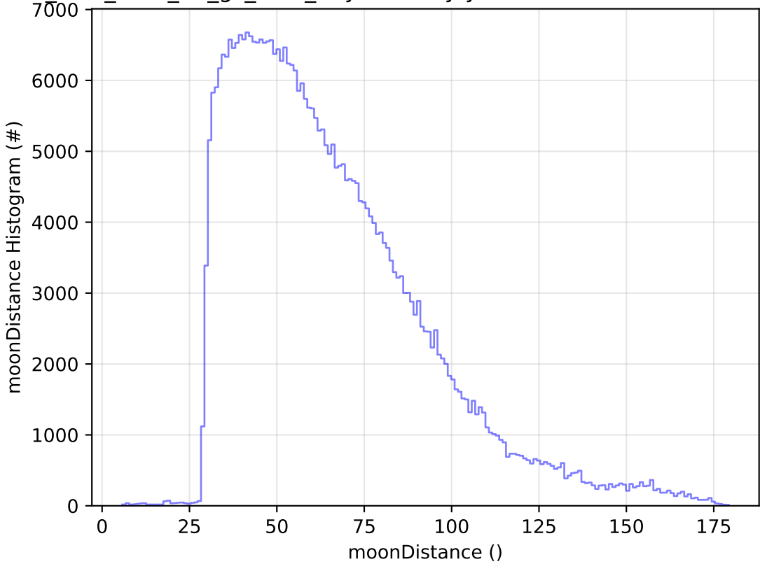
too_elab_r128_d2_gz_v3.4_10yrs All sky y band: moonDistance Histogram
