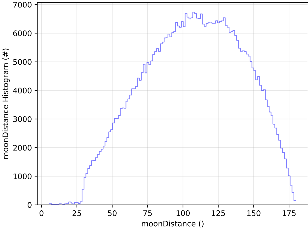
too_elab_r128_d2_gz_v3.4_10yrs All sky r band: moonDistance Histogram
