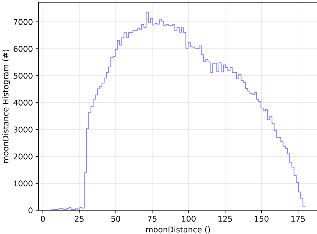
too_elab_r128_d2_gz_v3.4_10yrs All sky i band: moonDistance Histogram
