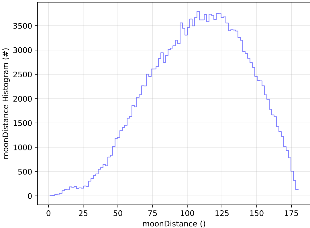
too_elab_r128_d2_gz_v3.4_10yrs All sky g band: moonDistance Histogram
