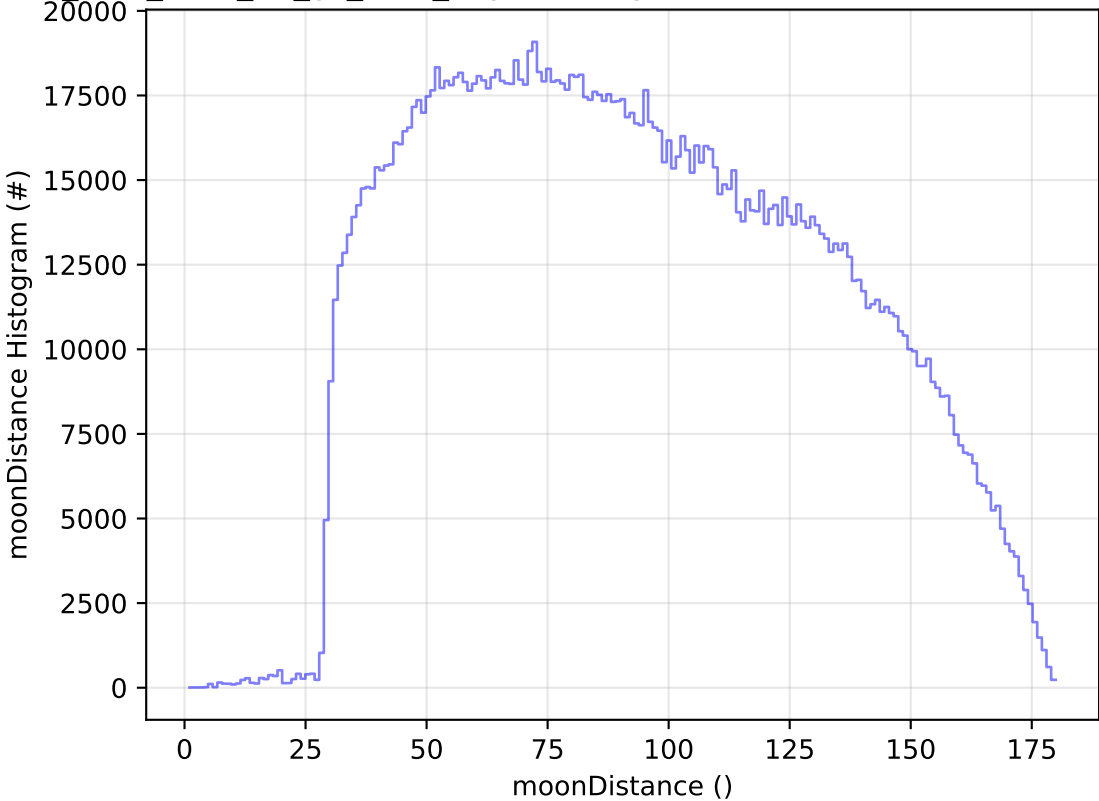
too_elab_r128_d2_gz_v3.4_10yrs All sky all bands: moonDistance Histogram
