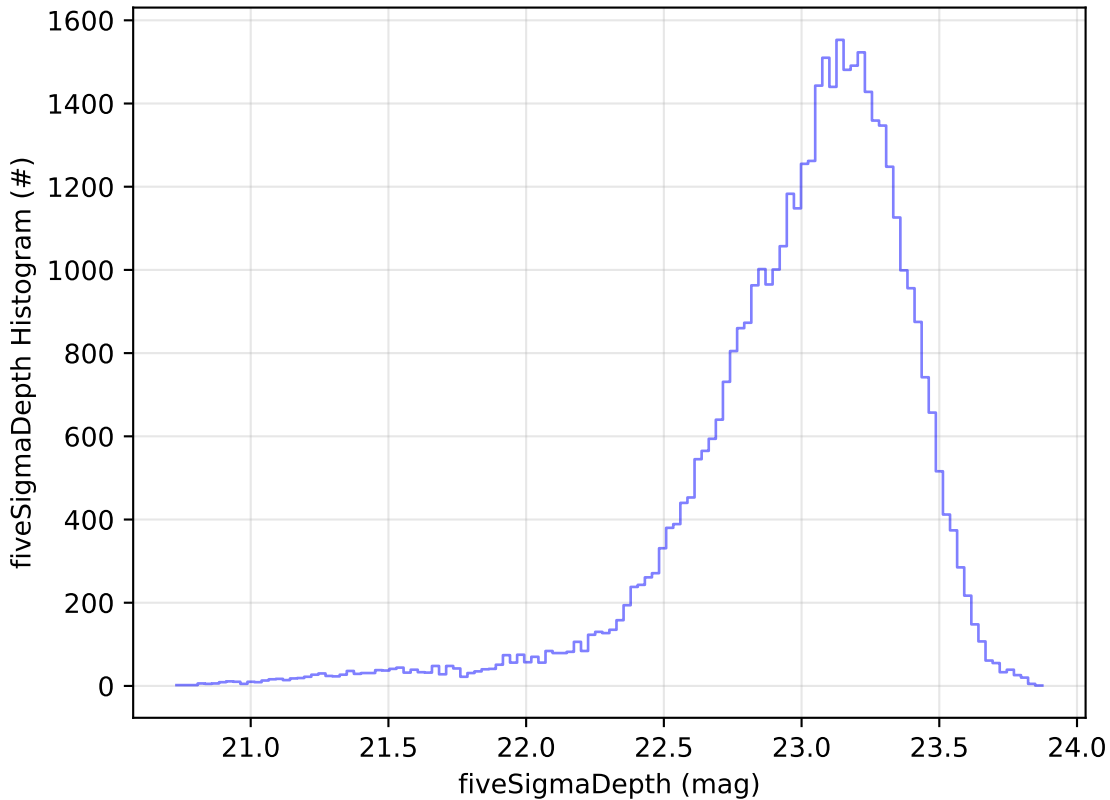
too_elab_r128_d2_gz_v3.4_10yrs Yr 1 z band: fiveSigmaDepth Histogram
