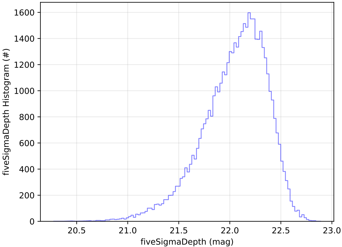
too_elab_r128_d2_gz_v3.4_10yrs Yr 1 y band: fiveSigmaDepth Histogram
