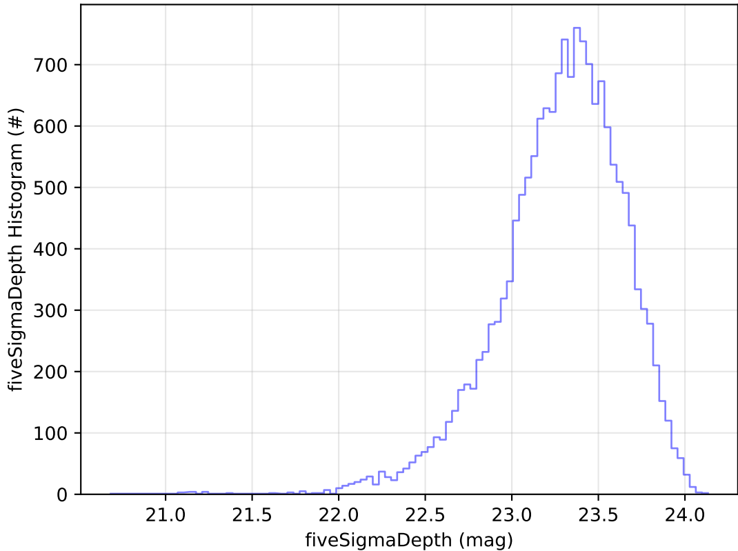
too_elab_r128_d2_gz_v3.4_10yrs Yr 1 u band: fiveSigmaDepth Histogram
