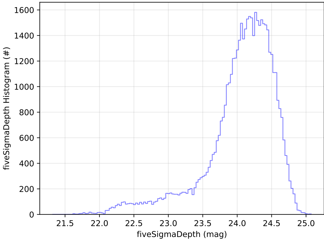
too_elab_r128_d2_gz_v3.4_10yrs Yr 1 r band: fiveSigmaDepth Histogram
