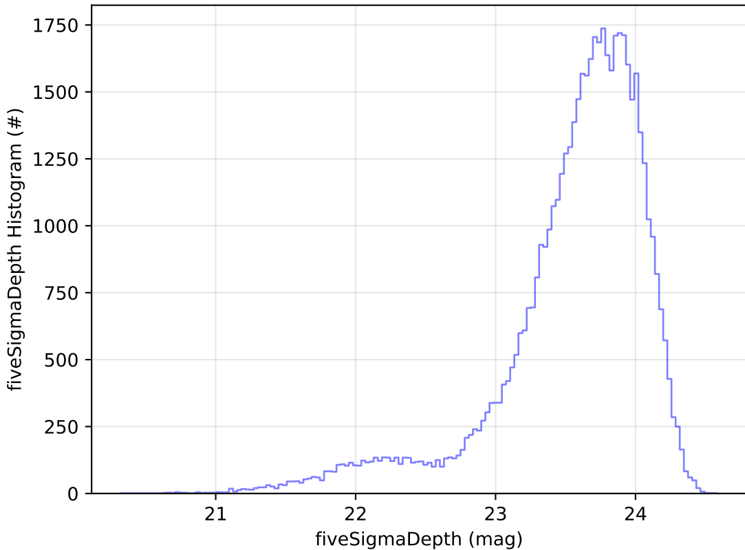
too_elab_r128_d2_gz_v3.4_10yrs Yr 1 i band: fiveSigmaDepth Histogram
