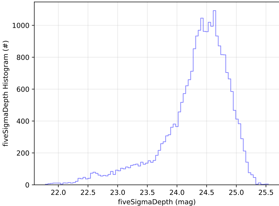
too_elab_r128_d2_gz_v3.4_10yrs Yr 1 g band: fiveSigmaDepth Histogram
