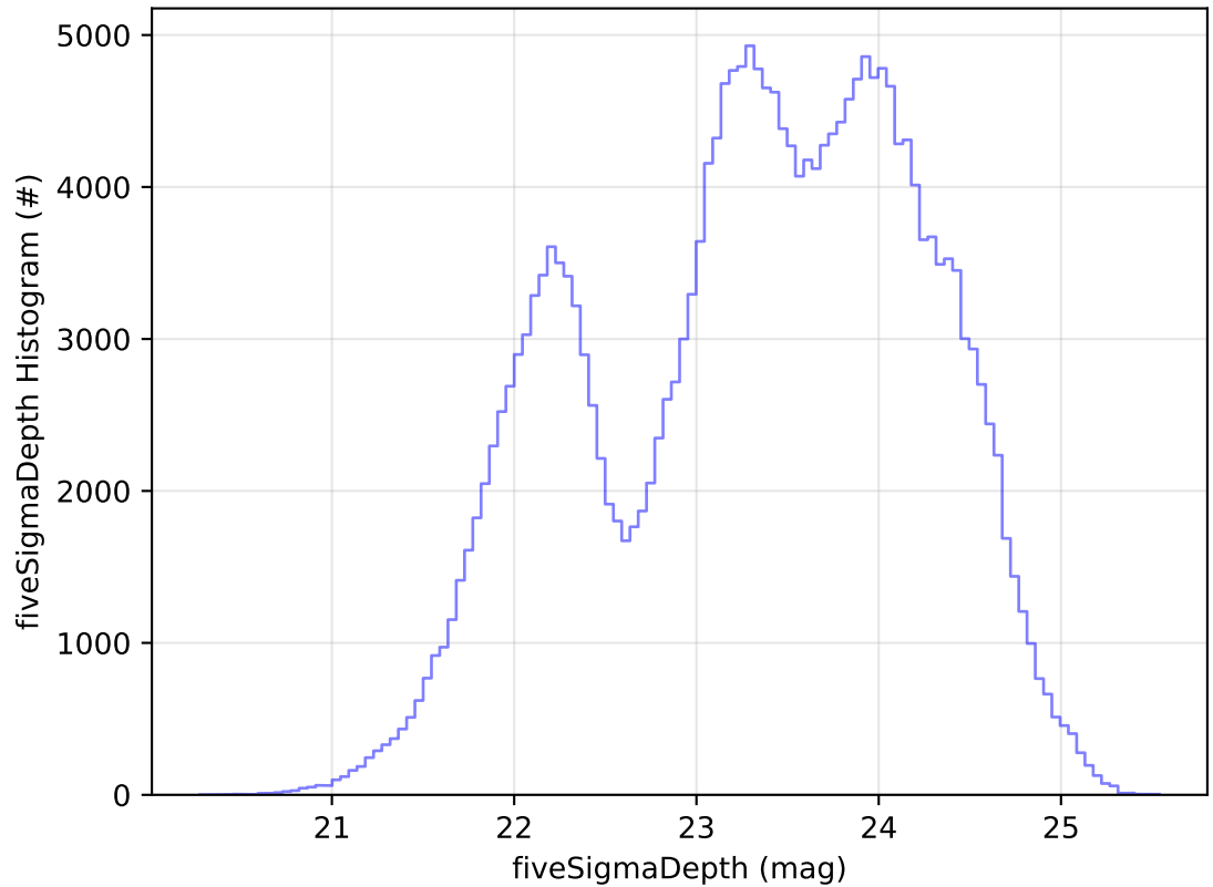
too_elab_r128_d2_gz_v3.4_10yrs Yr 1 all bands: fiveSigmaDepth Histogram
