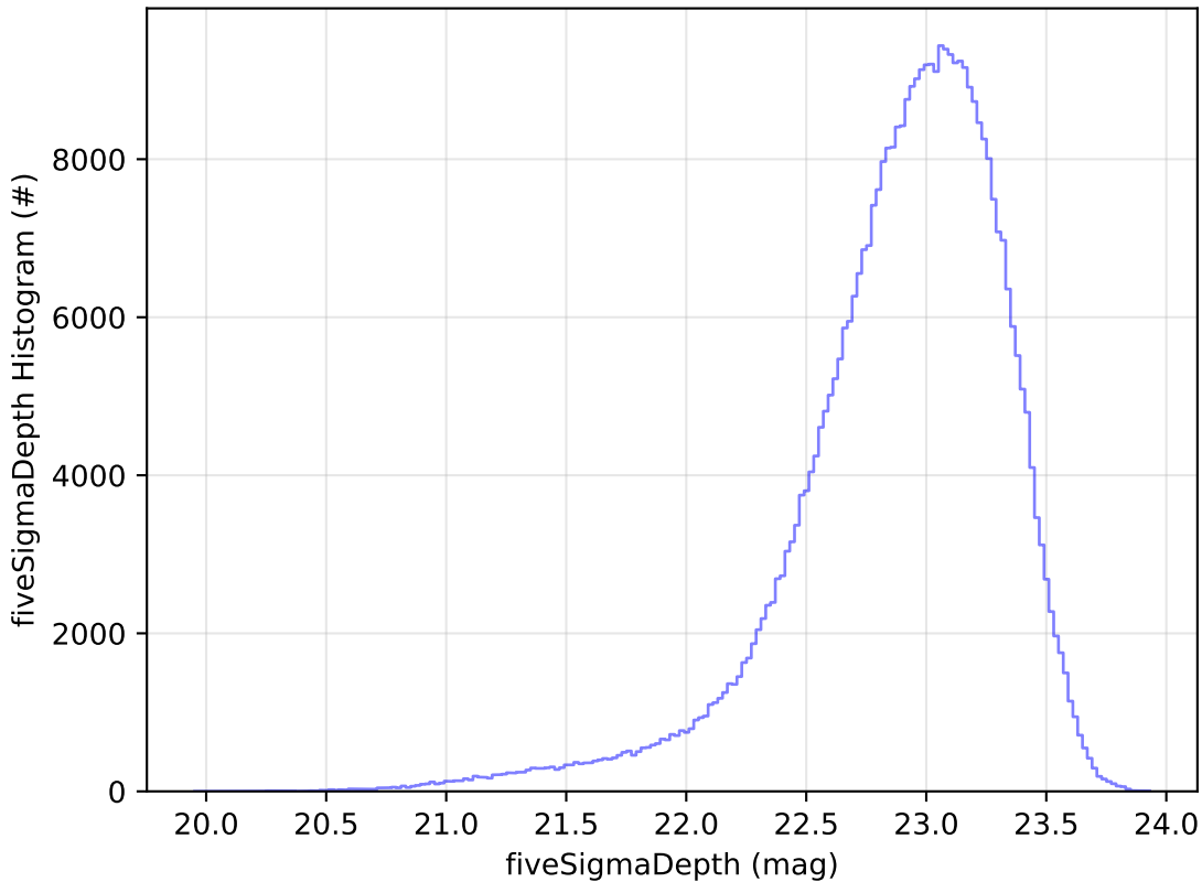
too_elab_r128_d2_gz_v3.4_10yrs WFD z band: fiveSigmaDepth Histogram
