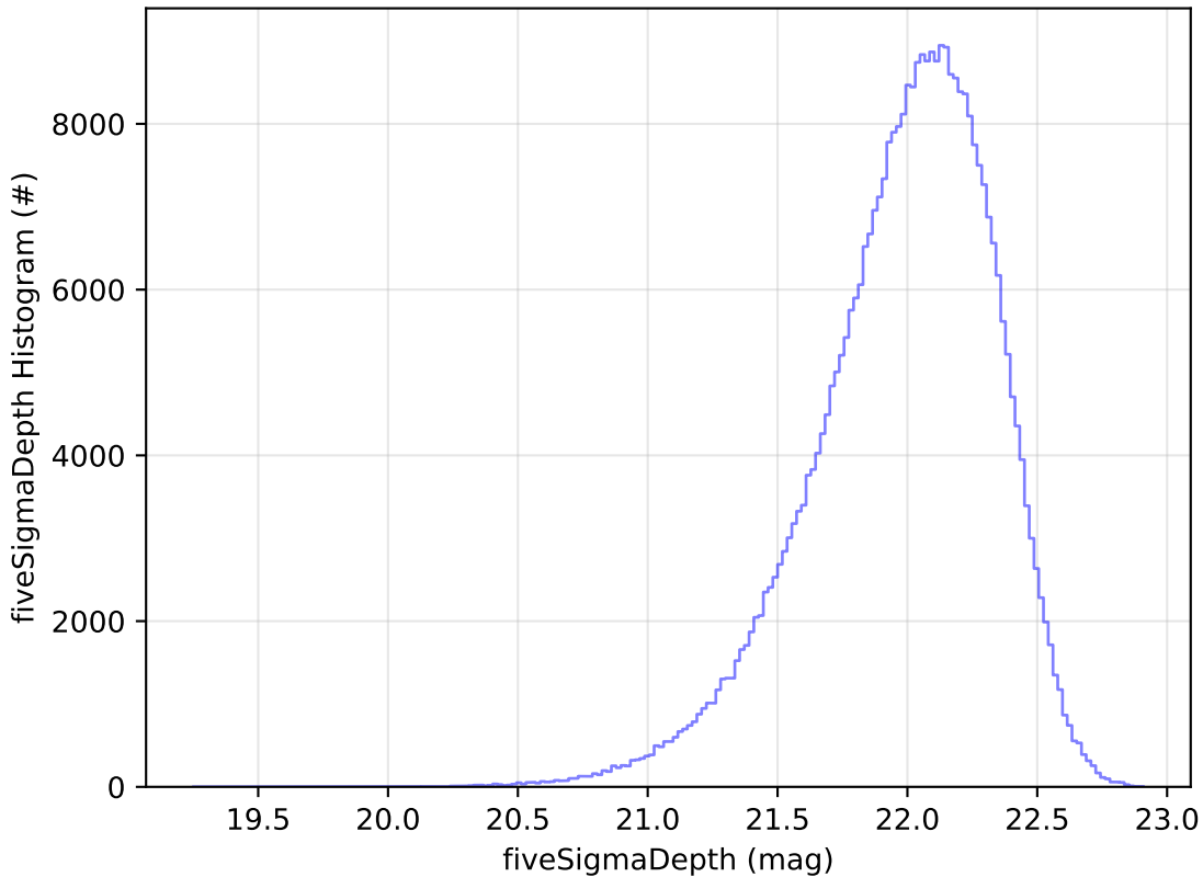
too_elab_r128_d2_gz_v3.4_10yrs WFD y band: fiveSigmaDepth Histogram
