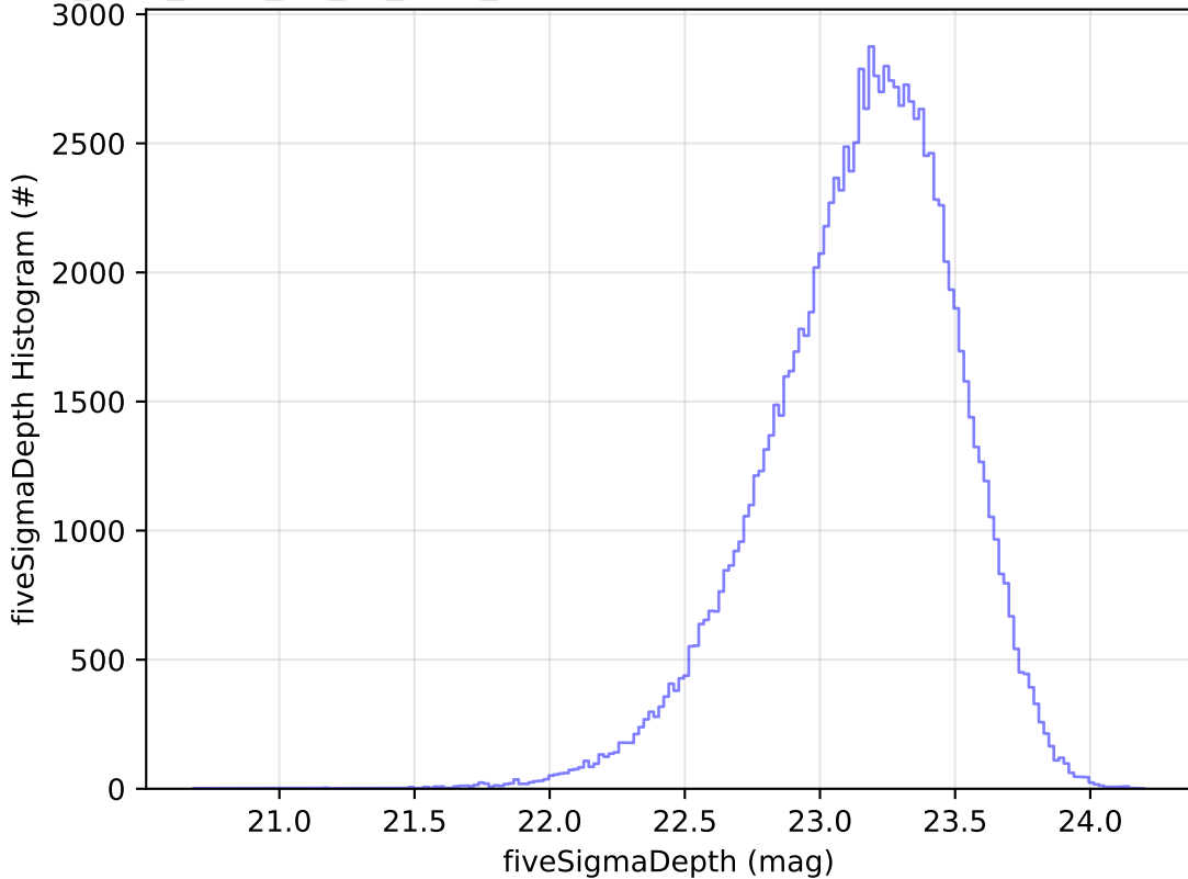
too_elab_r128_d2_gz_v3.4_10yrs WFD u band: fiveSigmaDepth Histogram
