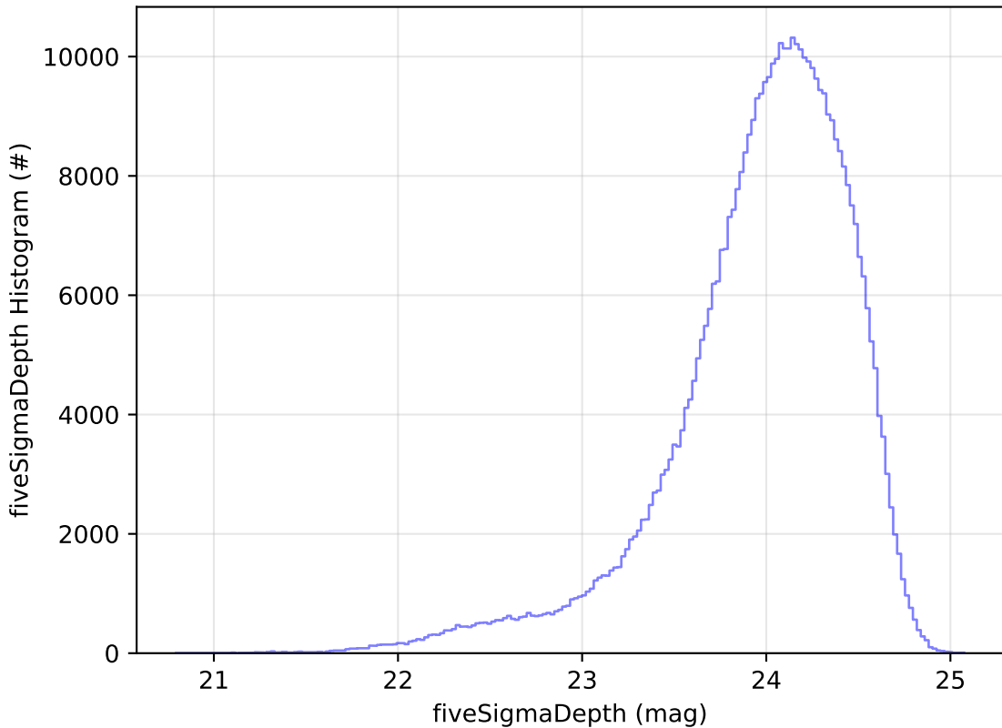
too_elab_r128_d2_gz_v3.4_10yrs WFD r band: fiveSigmaDepth Histogram
