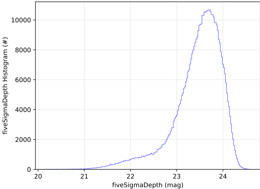
too_elab_r128_d2_gz_v3.4_10yrs WFD i band: fiveSigmaDepth Histogram
