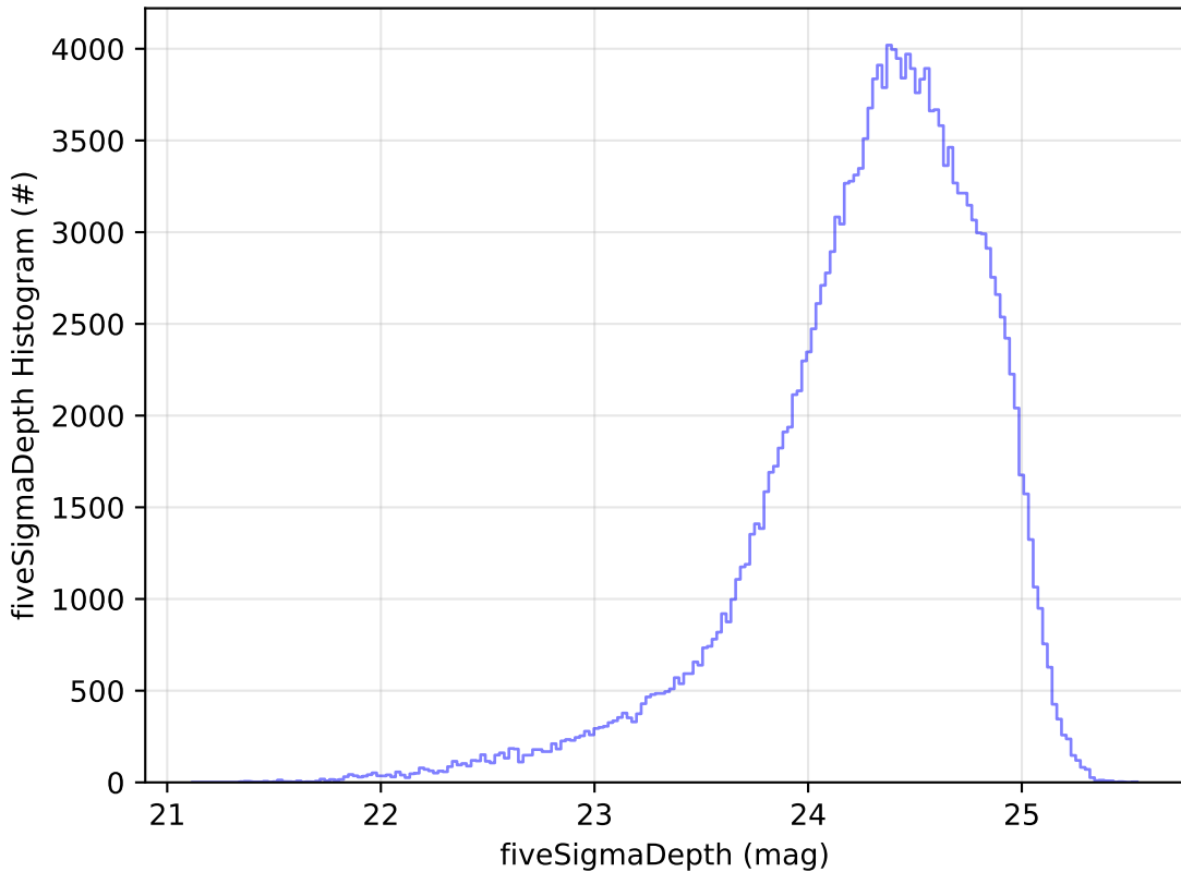
too_elab_r128_d2_gz_v3.4_10yrs WFD g band: fiveSigmaDepth Histogram
