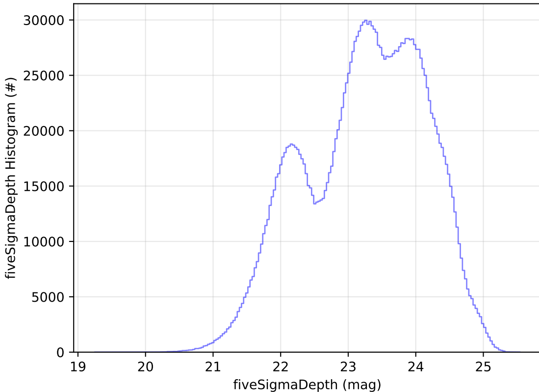
too_elab_r128_d2_gz_v3.4_10yrs WFD all bands: fiveSigmaDepth Histogram
